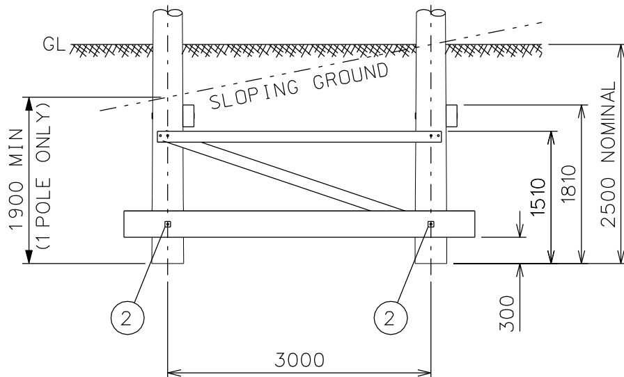
FRONT ELEVATION
